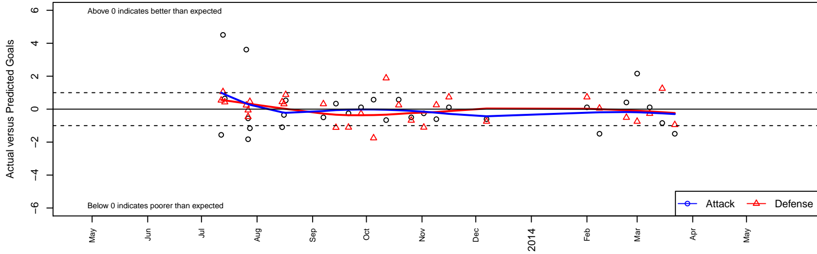
Cascade FC G02 Dots are actual minus expected GF (blue circles) and GA (red triangles). Blue line is smoothed change in attack strength. Red is smoothed change in defense strength.
